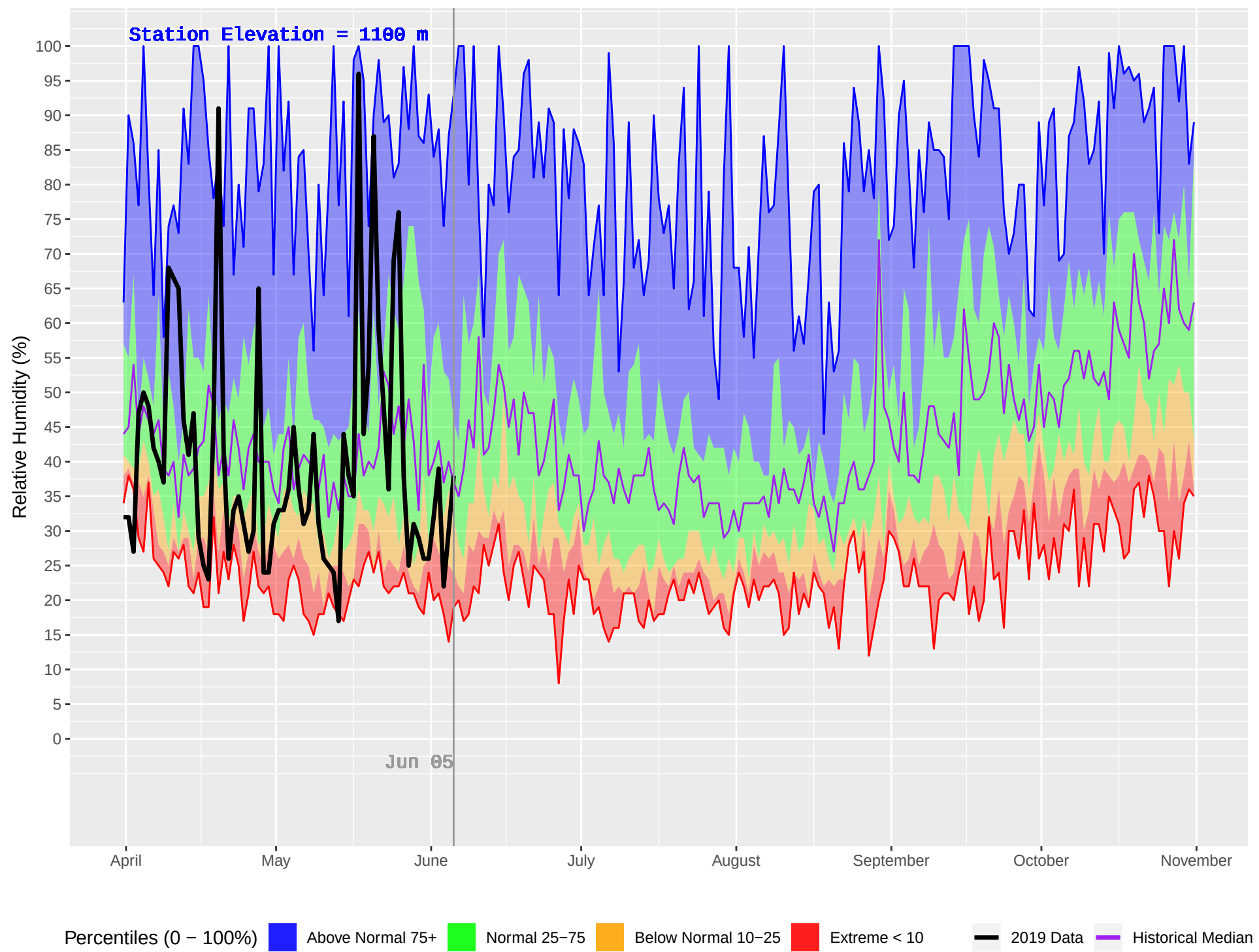
CHURN CREEK (832) : Historical (2003–2018) and Current (2019) Daily Relative Humidity
