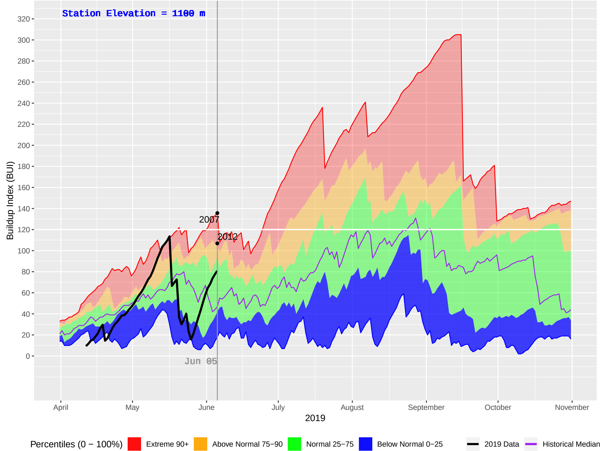
CHURN CREEK (832) : Historical (2003–2018), Current (2019) Daily Buildup Index (BUI)
