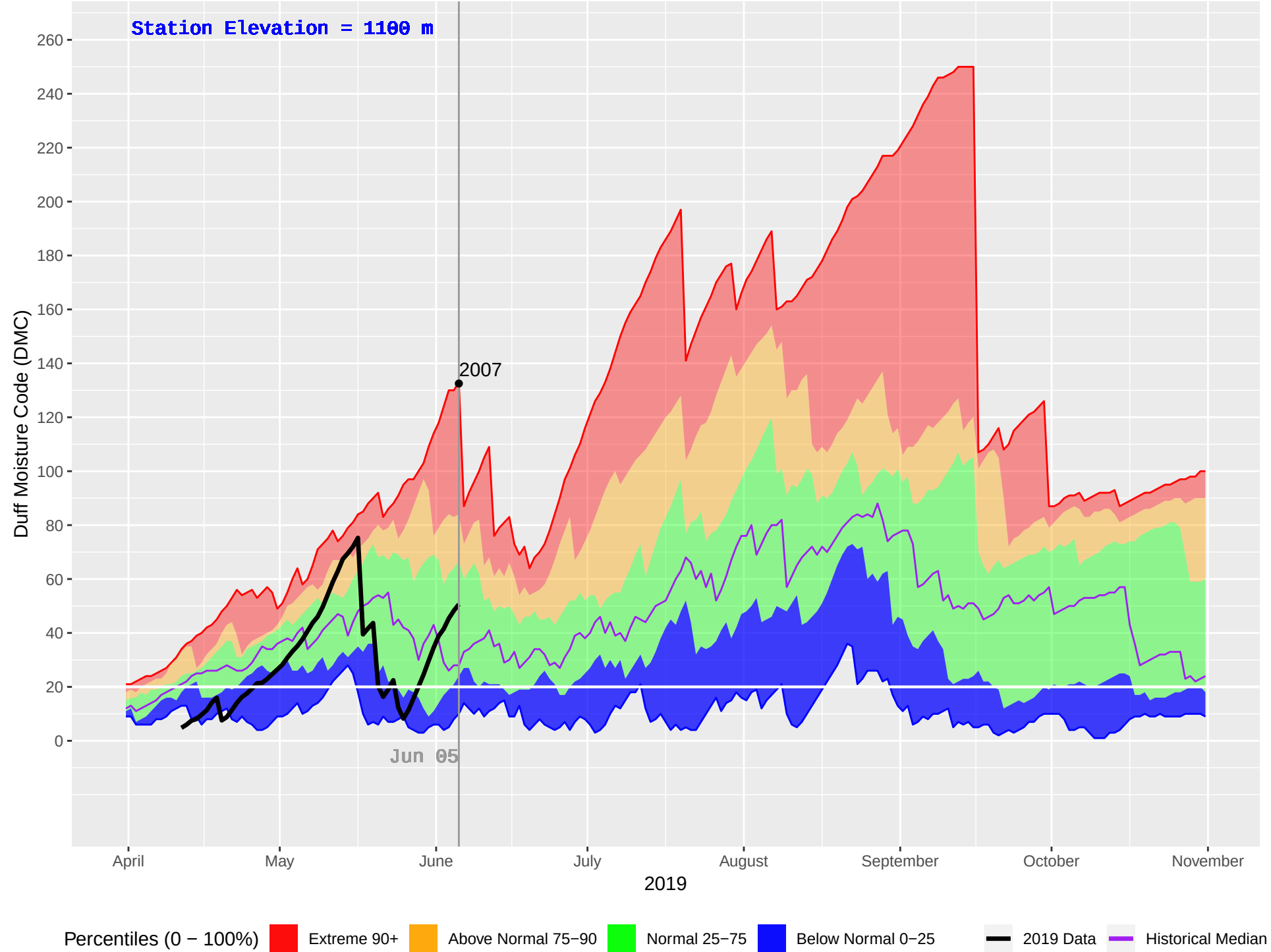
CHURN CREEK (832) : Historical (2003–2018), Current (2019) Daily Duff Moisture Code (DMC)
