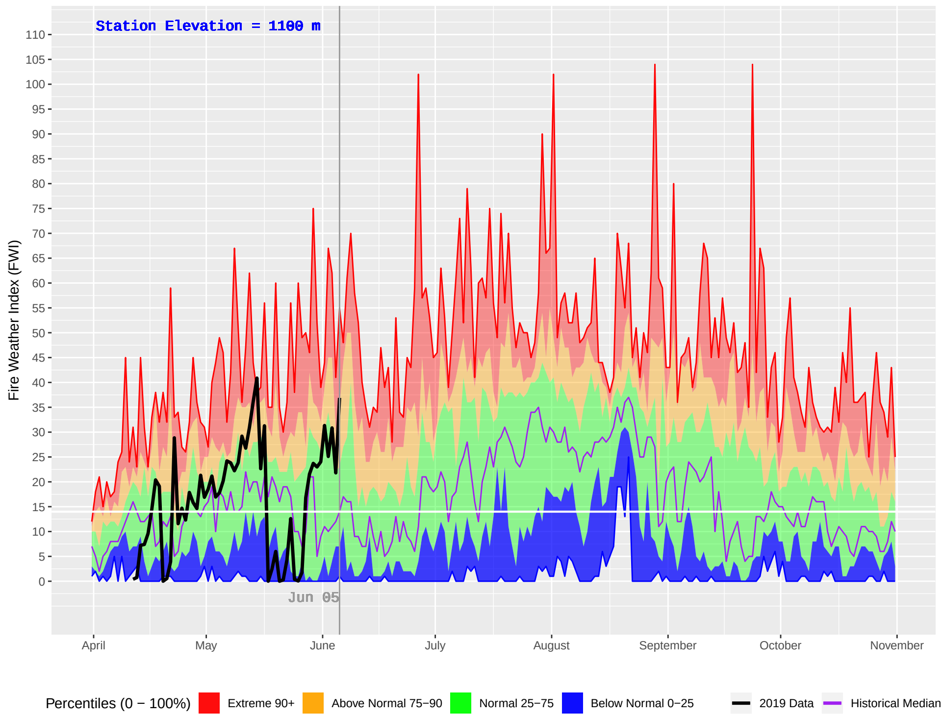
CHURN CREEK (832) : Historical (2003–2018) and Current (2019) Daily Fire Weather Index (FWI)
