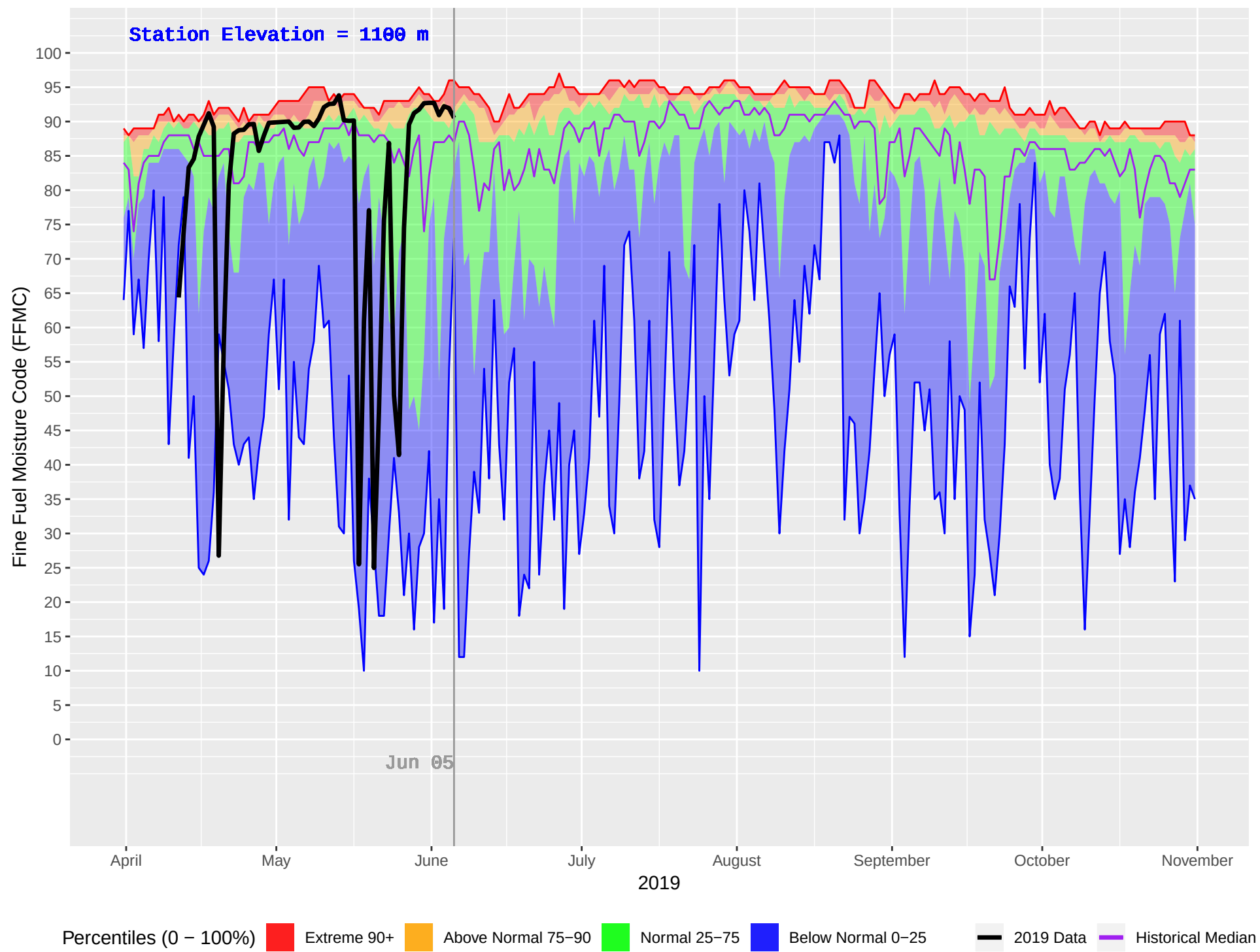
CHURN CREEK (832) : Historical (2003–2018) and Current (2019) Daily Fine Fuel Moisture Code (FFMC)
