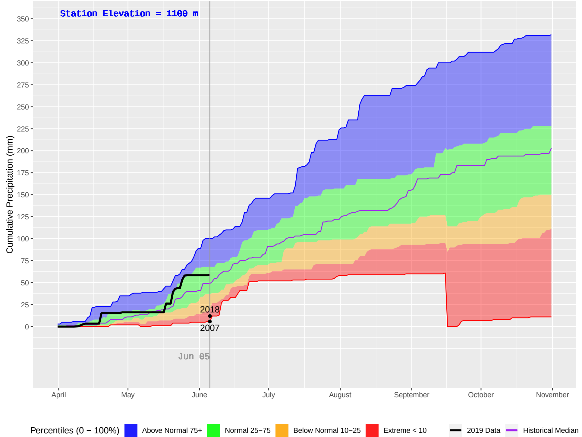
CHURN CREEK (832) : Historical (2003–2018), Current (2019) Daily Cumulative Precipitation
