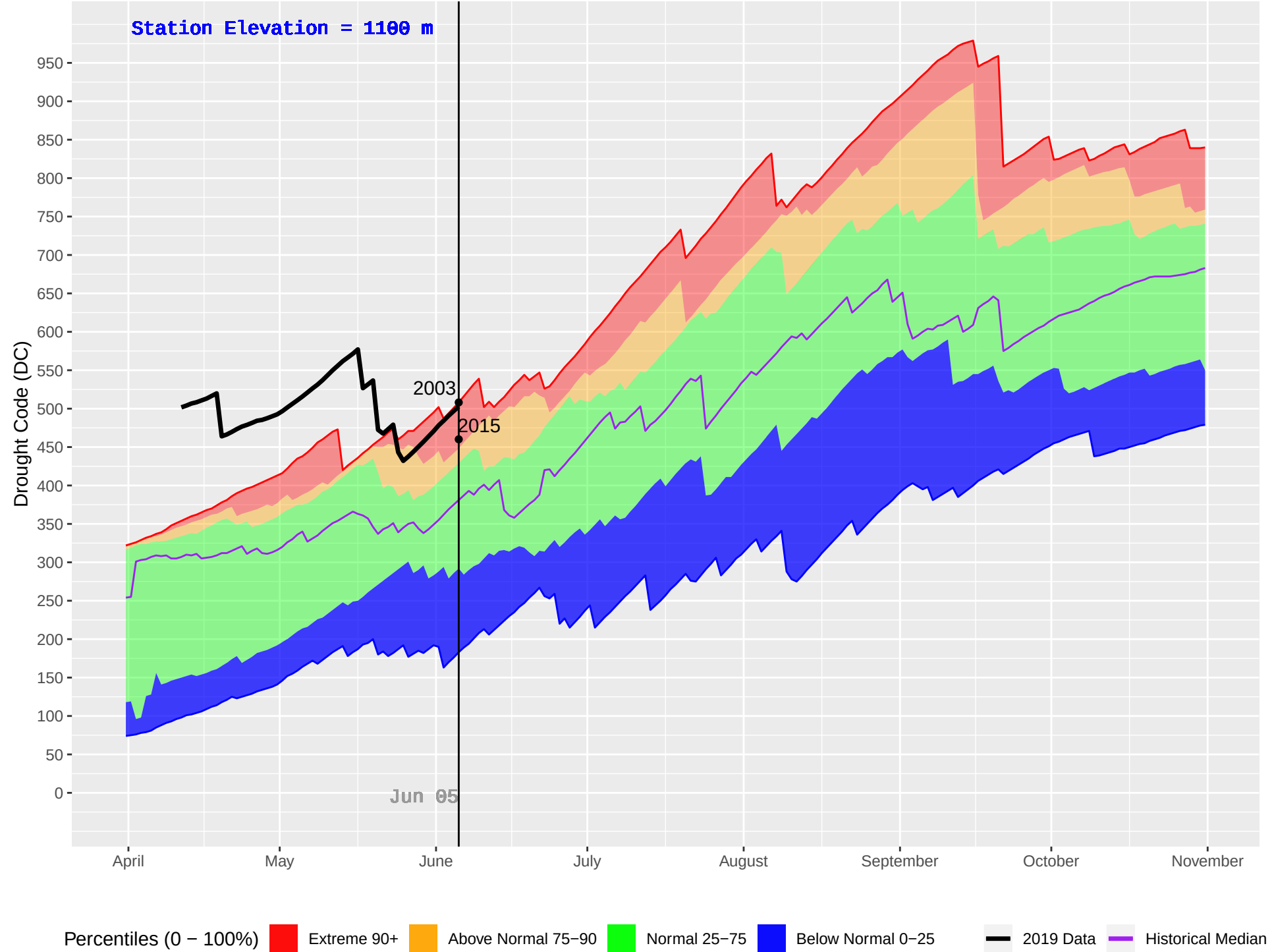
CHURN CREEK (832) : Historical (2003–2018) and Current (2019) Daily Drought Code (DC)
